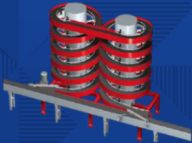
ACCUMULATOR BUFFER CONVEYOR
